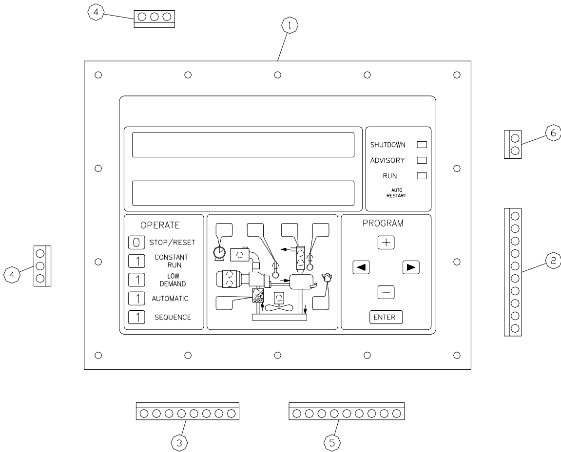
327EAU810-B (Ref. Drawing)
