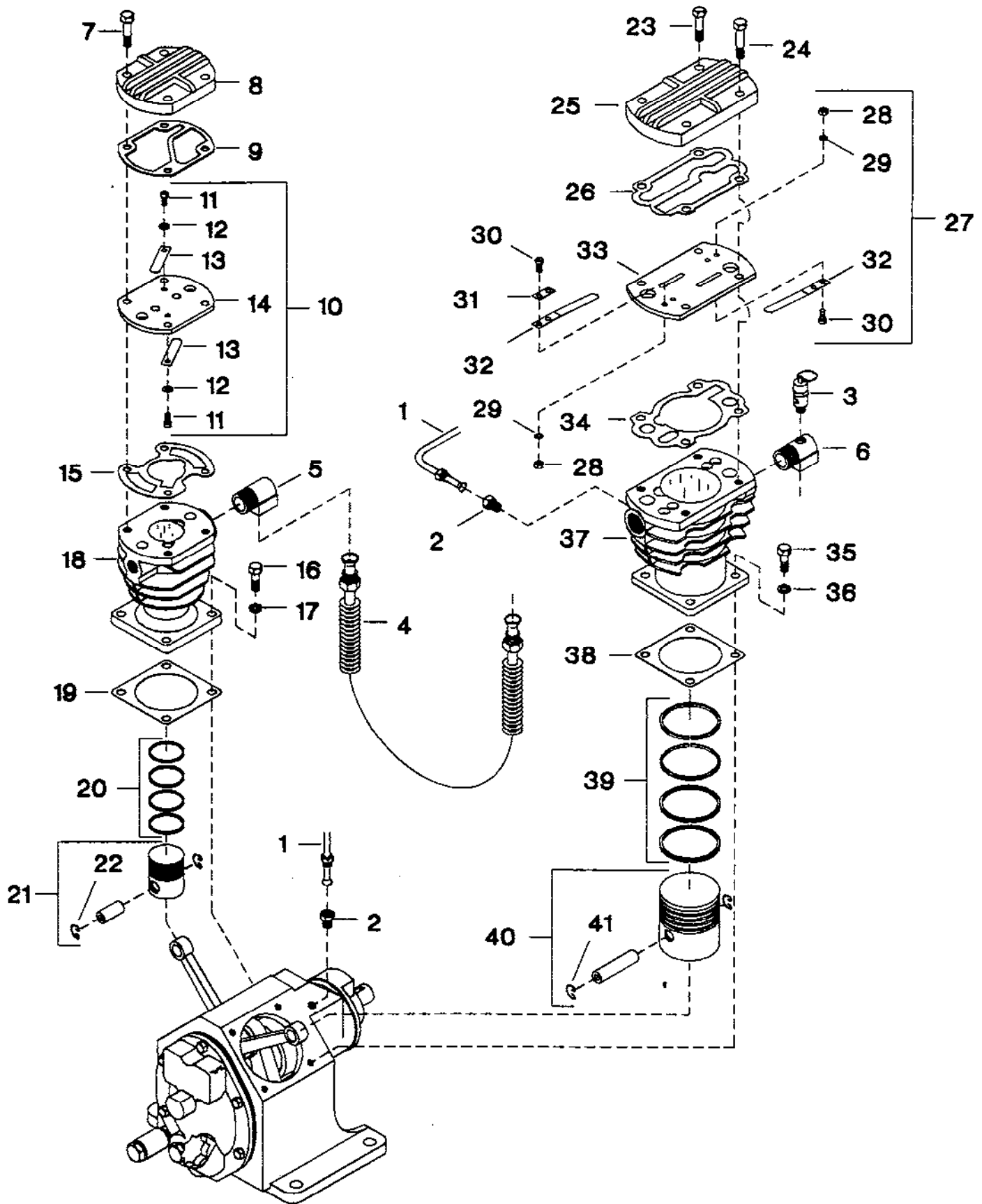
FIGURE 2. MODEL 234 COMPRESSOR, 1ST AND 2ND STAGE CYLINDER
