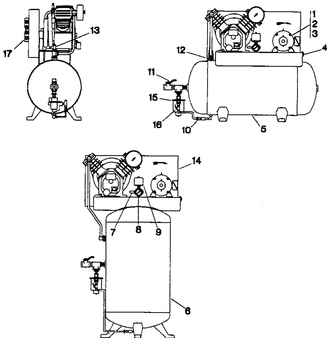
FIGURE 3. TYPICAL COMPRESSOR DRIVE, RECEIVERS AND ACCESSORIES
