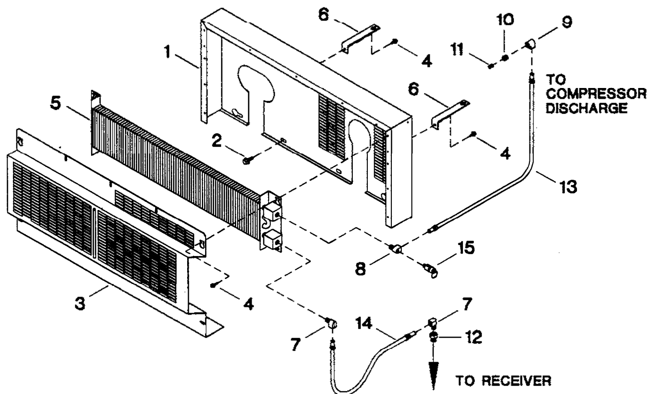
FIGURE 4. AIR COOLED AFTERCOOLER
