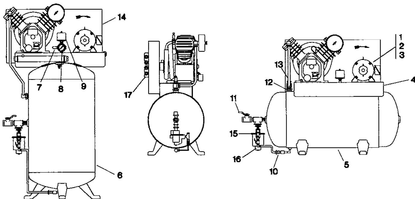
FIGURE 4. TYPICAL COMPRESSOR DRIVE, RECEIVERS AND ACCESSORIES
