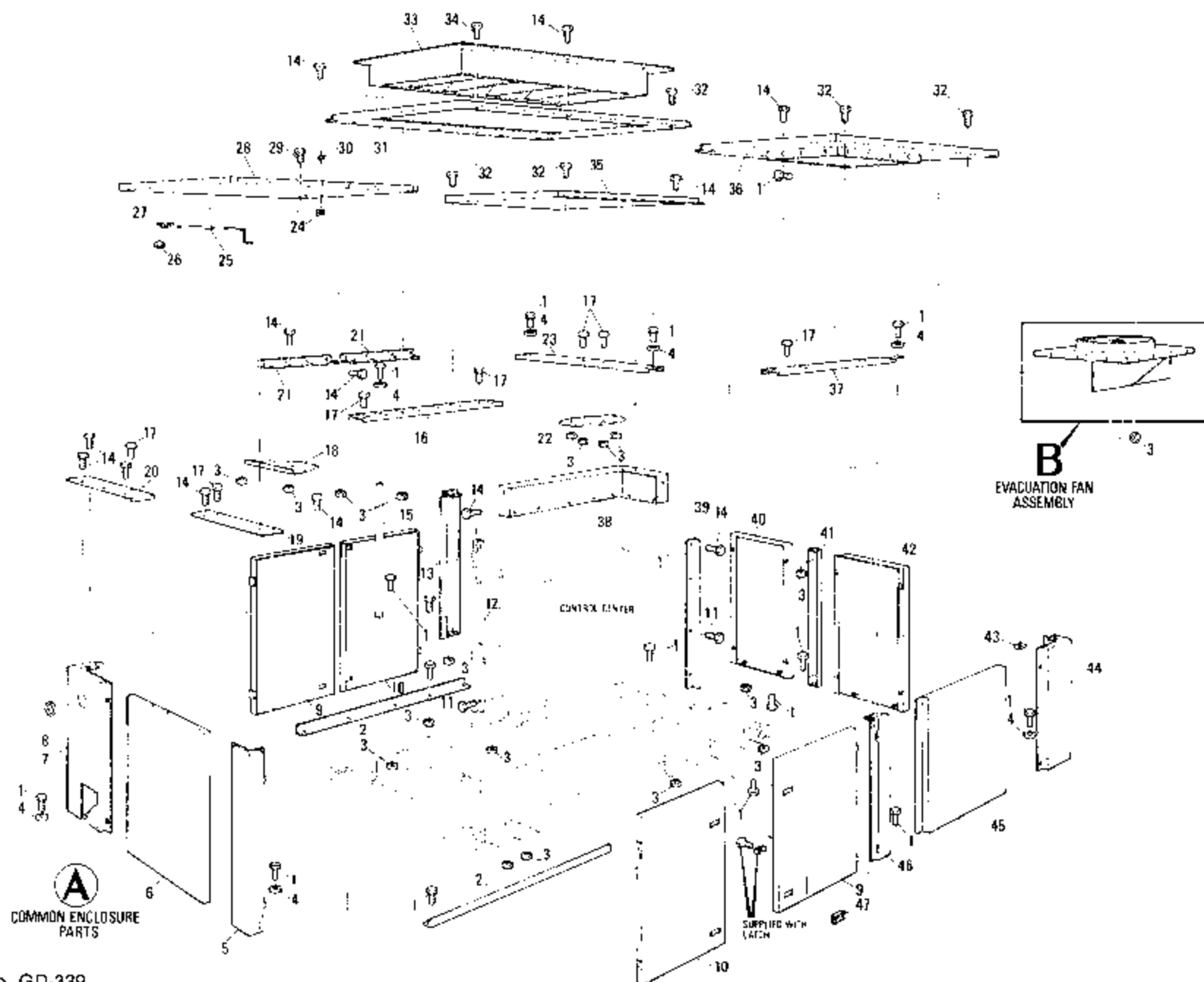
Drawing No. GD-339 Enclosure and Mounting Parts
