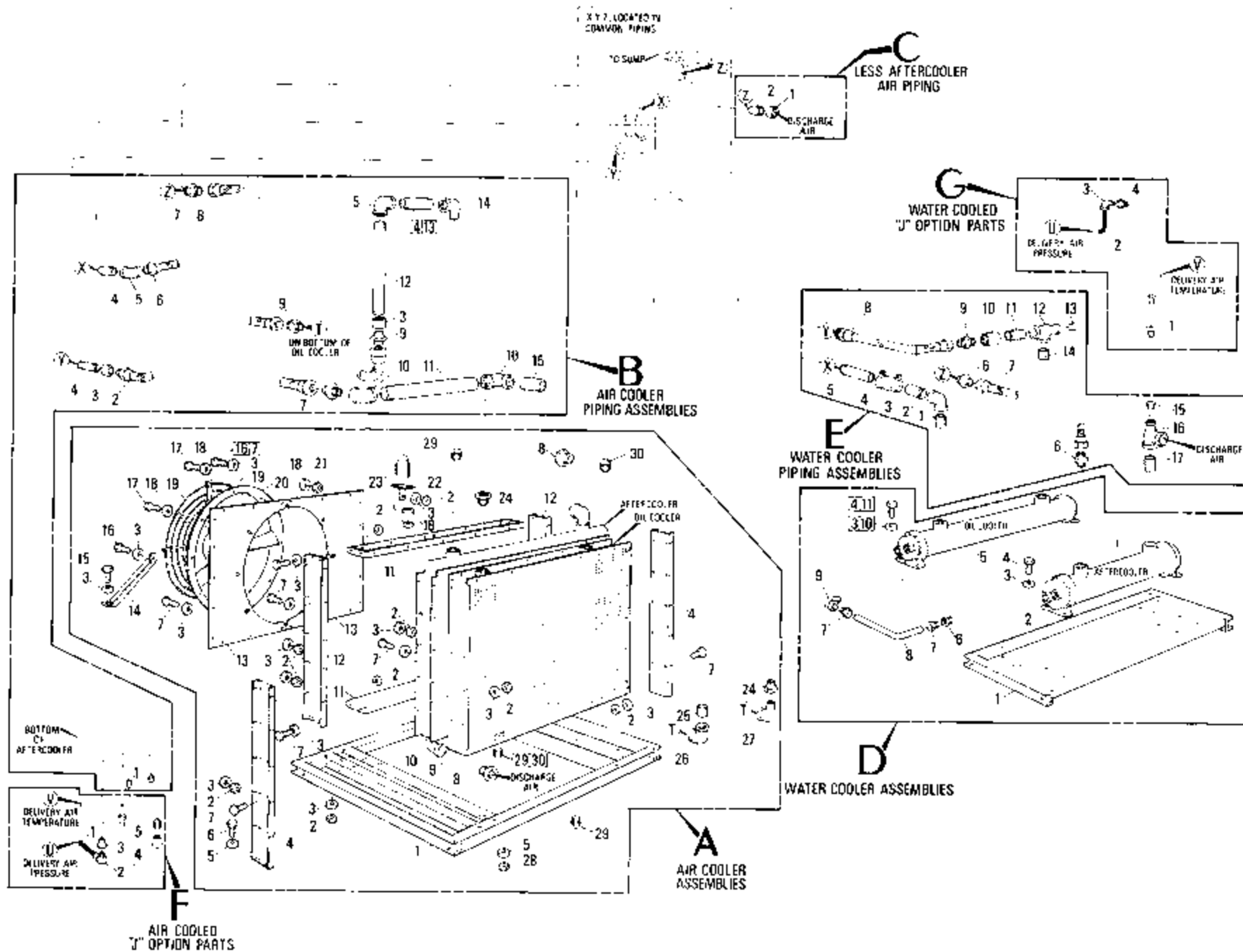
Drawing No. GD-337 Cooler and Piping Assemblies
